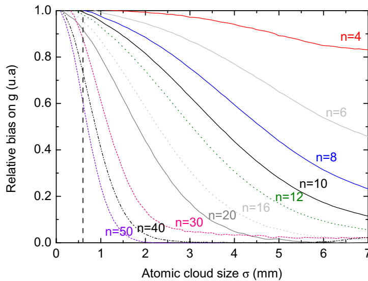
Figure 10. Relative bias on gravity measurements for an optical wave-front given by the Zernike polynomial Z_n^0 defined on a 30 mm radius disc, for different values of n . As n increases, the wave-front exhibits faster spatial variations, which are better averaged for large cloud sizes. All lines are normalized to the g bias calculated for an atomic cloud with \sigma = 0 . Vertical dashed line: measured initial atomic cloud size \sigma = 600 \mu\text{m} .
