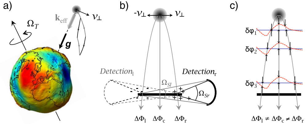
Figure 5. Systematic effects related to the cloud expansion. (a) Schematic representation of the Coriolis effect. For an atom with a nonzero transverse velocity v_{\perp} \neq 0 , a spatial area opens during the interferometer leading to a Sagnac phase shift. (b) Dispersion of the atoms position in the fluorescence detection zone due to the ballistic expansion. With a single-side collection optical system, Detection_r on the right, atoms with a velocity v_{\perp} have more impact on the measurement than those with a speed -v_{\perp} due to the difference in solid angles \Omega . Using a second system placed on the left restores the symmetry. (c) Propagation of the atomic cloud in an imperfect wave-front. For an atom whose trajectory is not perfectly vertical, the phases at the three pulses are different, leading to a systematic shift. The mean effect results from the convolution of this shift over the position and velocity distributions.
