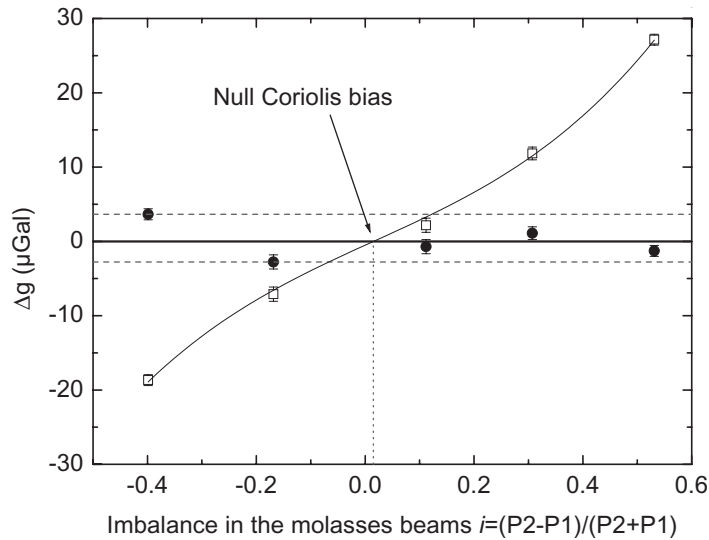
Figure 8. Combinations of the gravity values measured as a function of the imbalance in the molasses beams along the East–West direction and for two opposite orientations of the experiment. The white squares display half the difference in the signals, which corresponds to the Coriolis shift. The black circles display the half-sum and corresponds to the change in the other systematics that are all independent of the orientation of the experiment. They are dominated by the change in the wave-front aberration phase shift.
