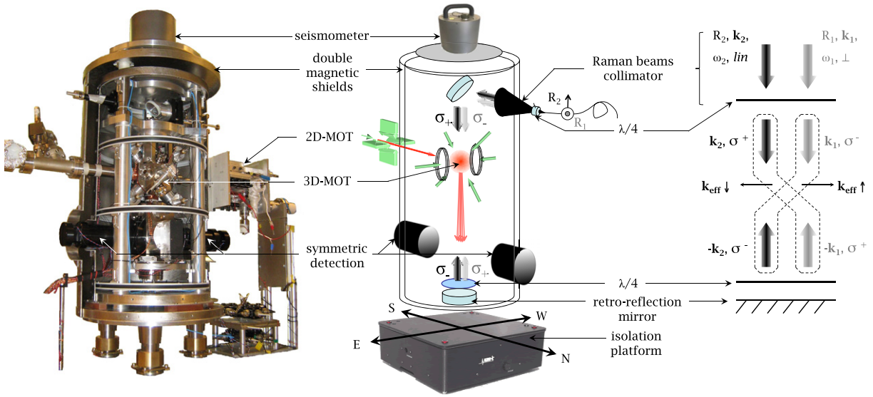
Figure 1. Left and center: photograph and schematic diagram of the cold atom gravimeter chamber with magnetic shields partially removed on the photograph (25 dB reduction). The 3D magneto-optical trap is in the upper area, composed of two horizontal beams in the East–West direction and four beams in the North–South plane. The free fall height is about 16 cm in a cylinder of diameter 40 mm from the 3D-MOT to the detection area at the bottom. In addition, a CCD camera (not represented) watches the 3D-MOT from the North–West. Right: configuration of the Raman laser beams. Two pairs of \sigma^-/\sigma^- and \sigma^+/\sigma^+ counter-propagating lasers allow us to induce Raman transitions with an effective wave vector k_{\text{eff}} pointing upwards or downwards. The Raman collimator aperture is 28 mm.
