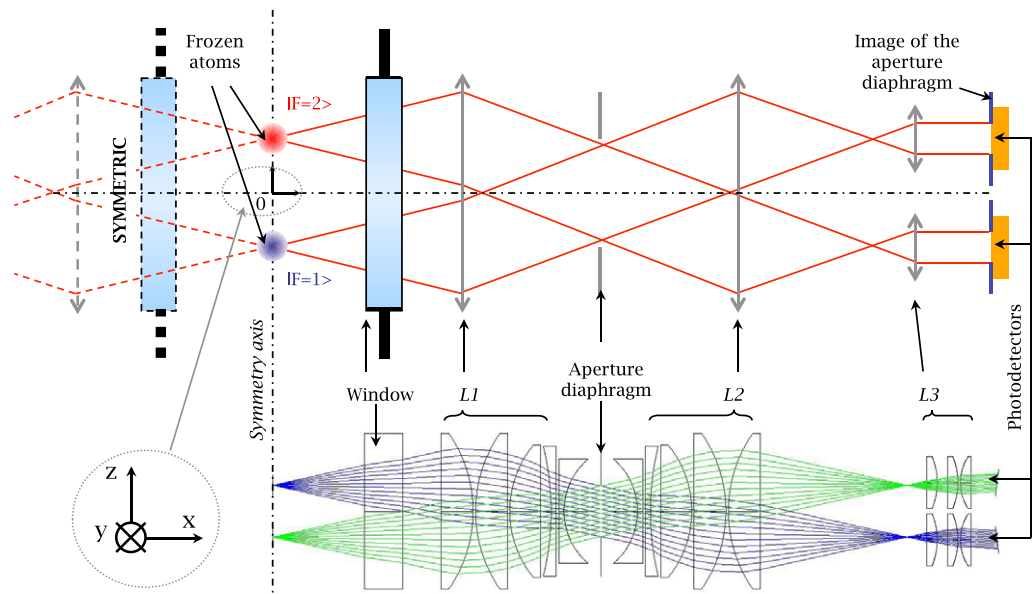
Figure 6. Optical setup for the collection of atomic fluorescence. The two atomic clouds are represented in red for |F = 2\rangle and in blue for |F = 1\rangle . The x - and y -axes correspond to the North–South and East–West directions, respectively.
