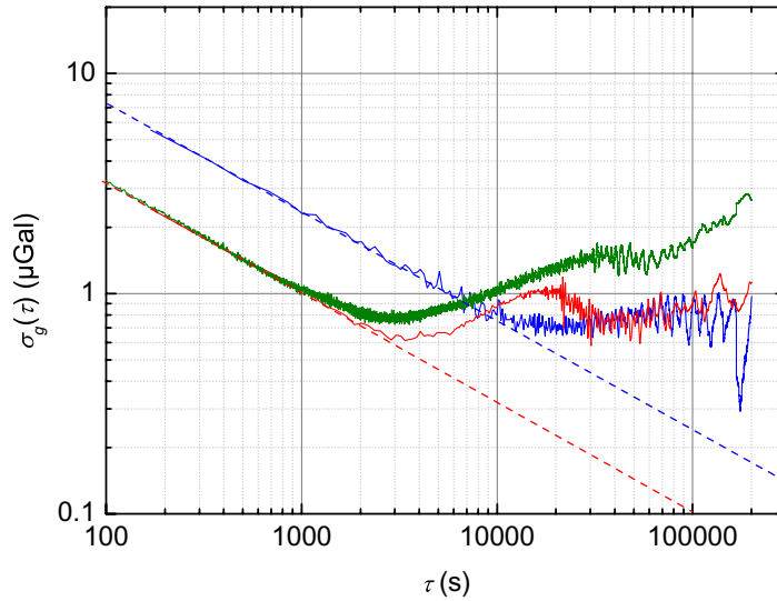
Figure 3. Allan standard deviation of the residual. Blue line: using the four-configuration algorithm to reject the LS2. Red and green lines: using only two configurations alternating k_{\uparrow} and k_{\downarrow} . Half-difference is represented in red and half-sum in green. They correspond to a red slope \sqrt{5/2} lower than the blue one.
