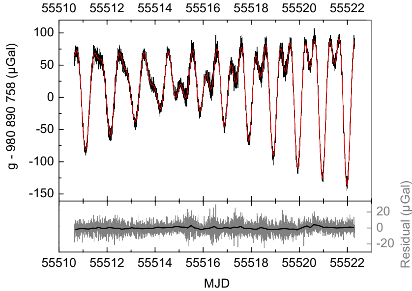
Figure 2. Top: continuous g measurement from 10 to 22 November 2010 uncorrected for tides (bins of 400 drops). Red solid line: tide model. Bottom: residuals, in gray for bins of 400 drops (170 s) and in black for bins of 10 000 s.
