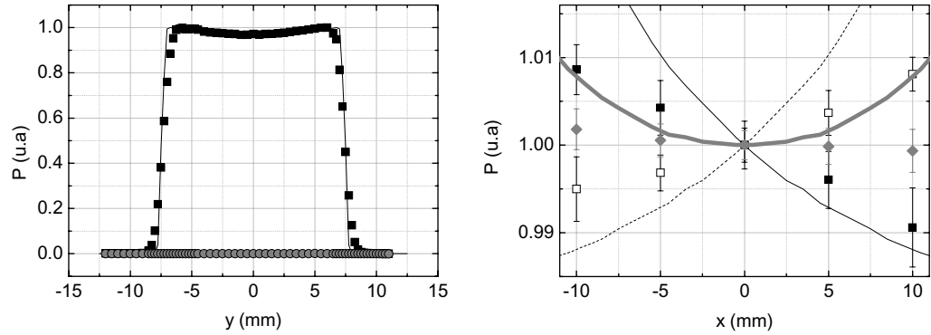
Figure 7. Study of the symmetry of the detection system. Normalized optical power measured on the photodiodes in the horizontal characterization. Left: the source is moved along the horizontal axis y , whereas z and x are constants such that the source is at the level of the center of a photodetector. Black squares and gray dots represent the experimental results for the two photodetectors of a single setup. Lines show the calculations with Zemax. Right: for both setups at the same z level as on the left for y = 0 . Black squares for the North setup and open squares for the South setup. Thin line: calculation with Zemax. Gray diamonds: half-sum of the measurements. Gray thick line: half-sum of the calculations.
