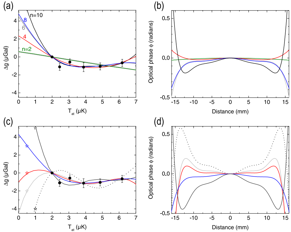
Figure 9. Black circles on (a) and (c): experimental values of g(T_{\text{at}}) - g(2\mu\text{K}) . (a) Fit to the data with subsets of Zernike polynomials ( Z_{n \leq n_{\text{max}}}^0 ) for increasing n_{\text{max}} . The linear fit, represented as a gray line, coincides with the fit corresponding to n_{\text{max}} = 2 . (b) Reconstructed wave-fronts. (c) Fits with the subset corresponding to n_{\text{max}} = 10 for different added fake points (stars) below 2\mu\text{K} . (d) Reconstructed wave-fronts.
