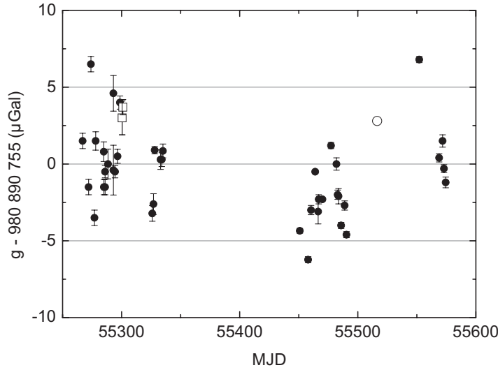
Figure 4. g absolute measurements from March 2010 to January 2011. The white circle corresponds to the measurement presented in figure 2. White squares present the measurements during the comparison in April 2010 [10]. The error bars represent the statistical uncertainties.
